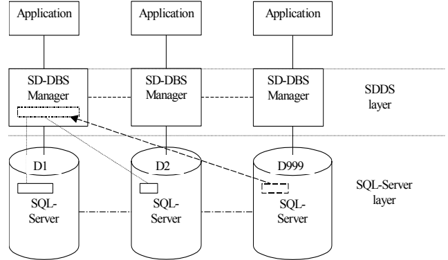
Fig. 1 Gross Architecture of SD-SQL Server
